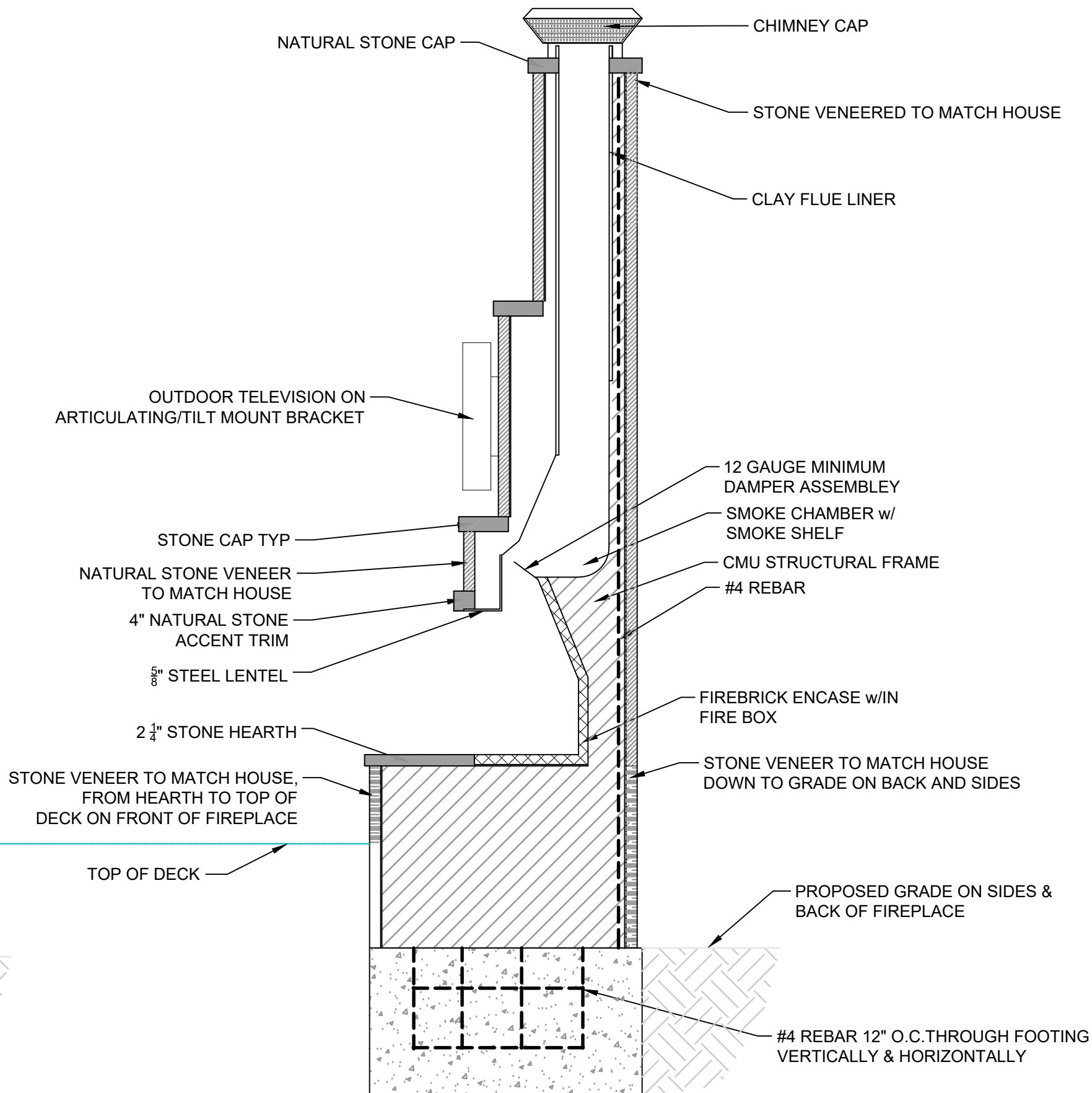
Cross section of fireplace
