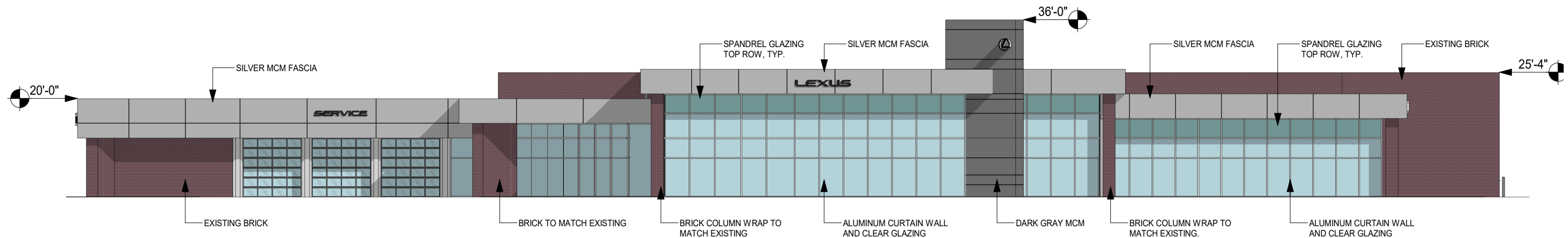
North Elevation 1" = 20'-0"
